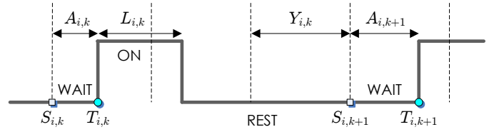
Fig. 2. User process Z_i(t) under NS-PCM, where dashed vertical lines represent bin boundaries.
