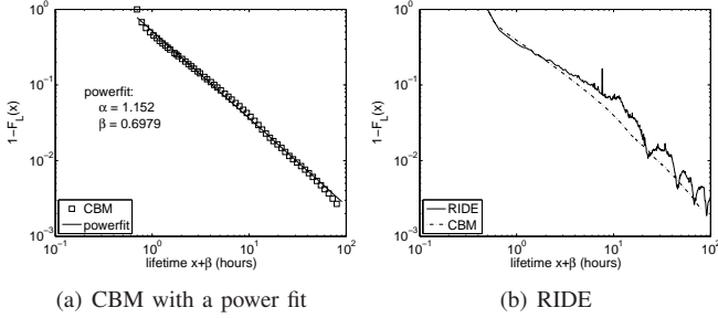
Fig. 7. Estimated lifetime distribution of all observed peers using CBM and RIDE.
