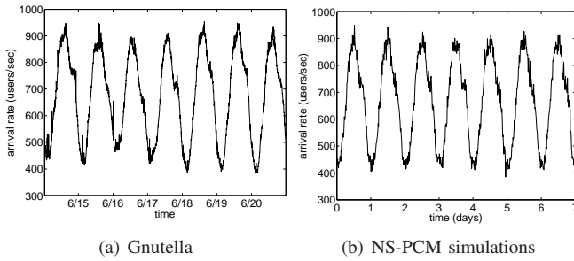
Fig. 3. User arrival rate: a) observed in Gnutella during June 14-20, 2007; b) obtained from NS-PCM simulations.
