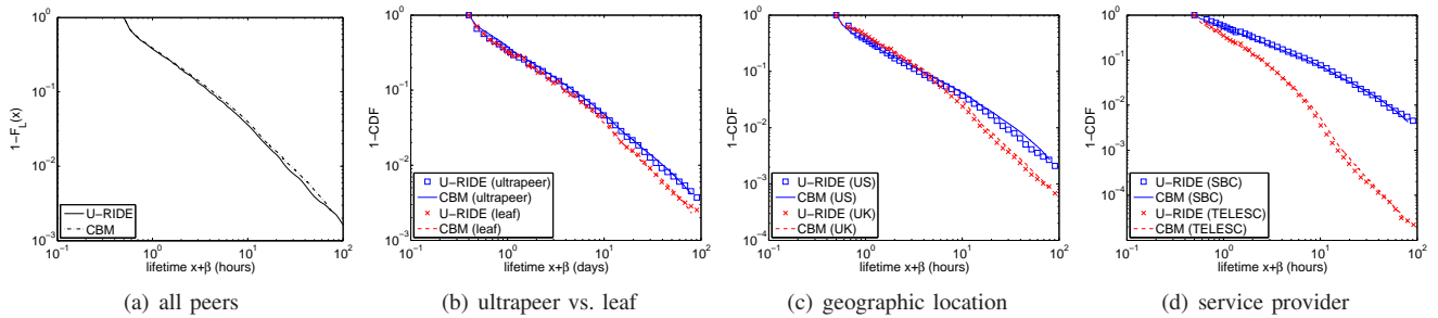
Fig. 8. Comparison of U-RIDE with CBM with M = 24, \epsilon_U = 1 in different datasets.
