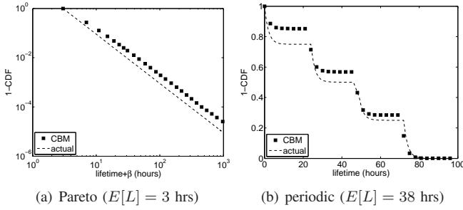
Fig. 4. CBM estimator (6) under NS-PCM.
