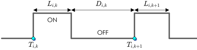
Fig. 1. User process Z_i(t) under SR-CM.
