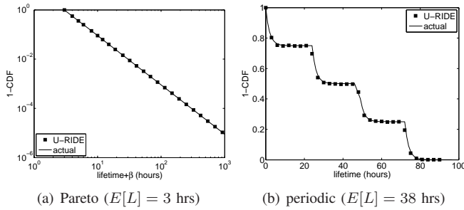
Fig. 6. U-RIDE estimator (17) with \mathcal{BS} under NS-PCM.
